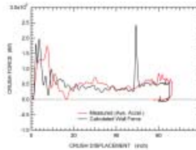
Crush Force Histories
